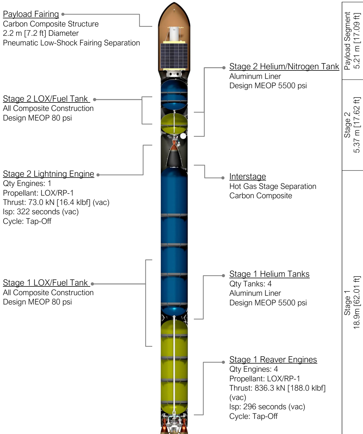
Figure 2. MK004 Alpha Launch Vehicle
