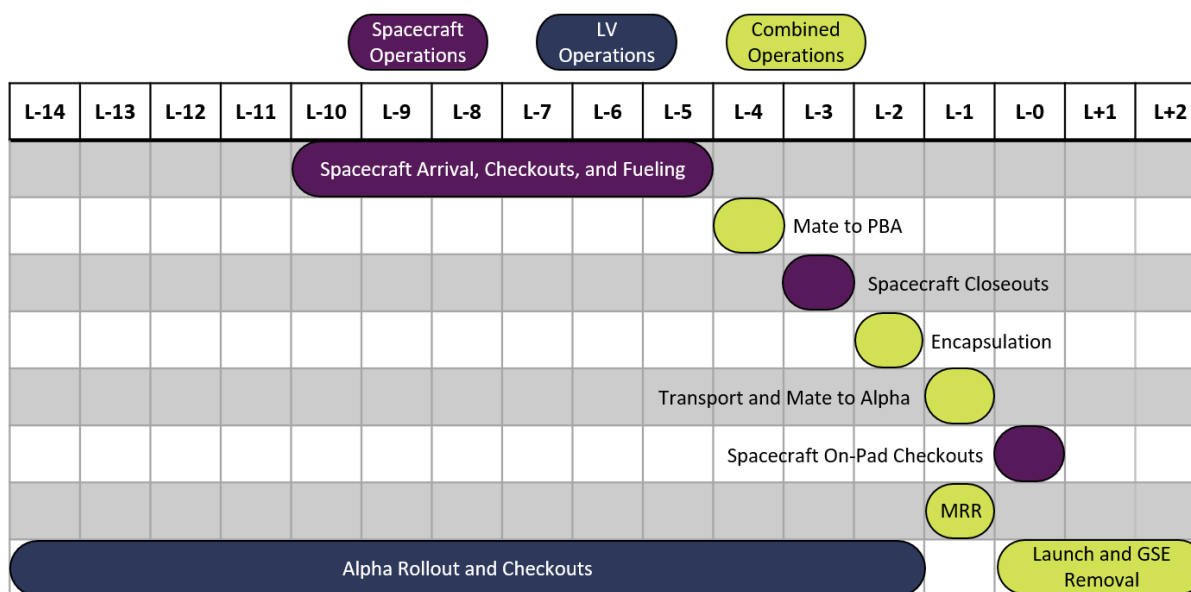
Figure 19. Nominal Payload Processing Flow
