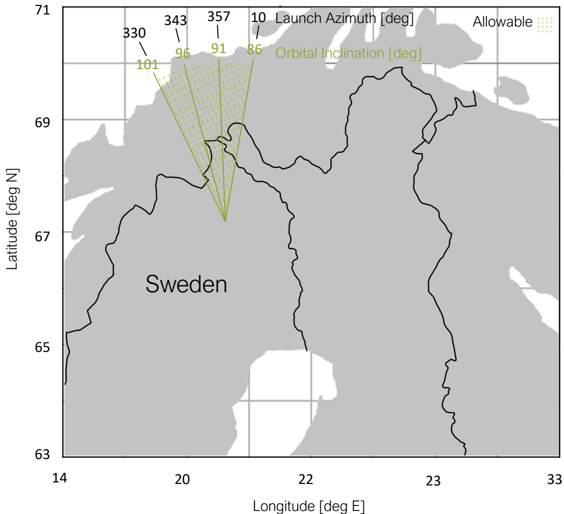
Figure 23. Esrange Space Center Launch Inclinations and Azimuths
