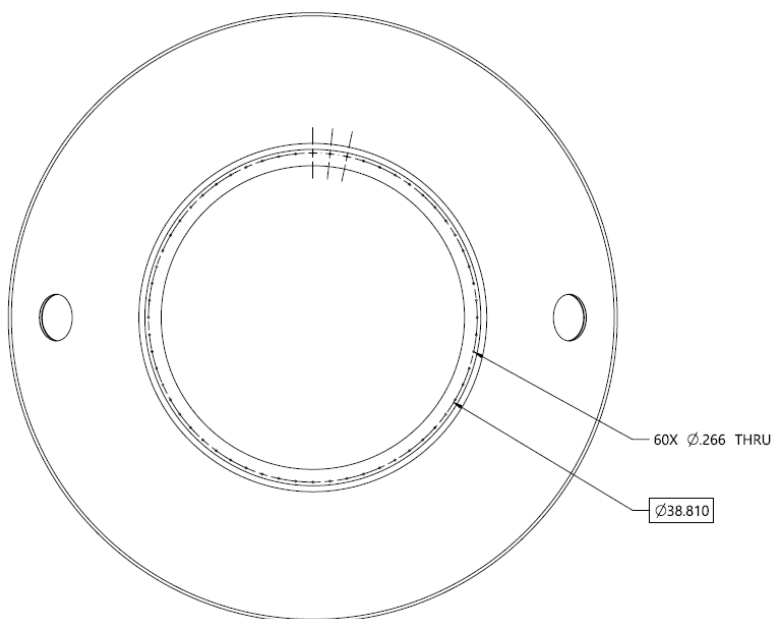
Figure 8. Payload Interface Dimensions in Launch Vehicle Coordinate Frame
